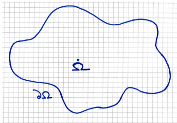
Figure 12: Domain of study \Omega for the Poisson equation \Delta w = \bar{f} . \mathring{\Omega} is its open interior, \partial\Omega is the outside boundary.
