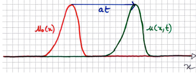
Figure 7: The initial profile u_0(x) is simply advected at velocity a .
